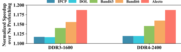
Fig. 16. Geomean IPC speedup with varying DRAM bandwidth.
